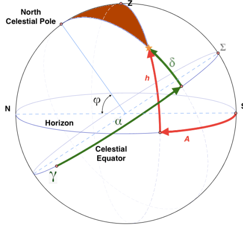
Figure 1.16: Conversion between horizontal and equatorial coordinate systems.
