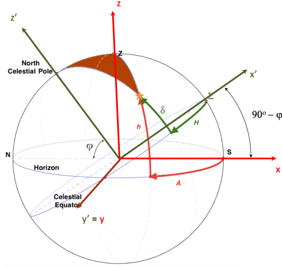
Figure 1.27: Hour and horizontal coordinates.
