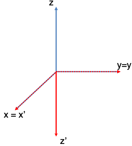
Figure 1.26: Right-handed system (blue) and left-handed system (red).
