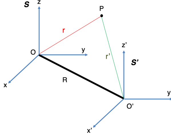
Figure 1.30: Coordinate translation.
