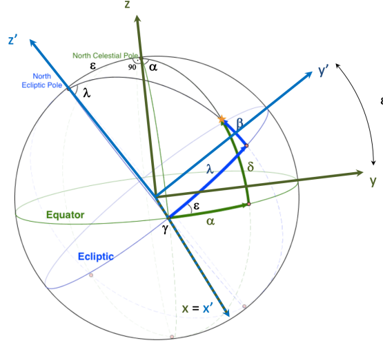
Figure 1.29: Equatorial and ecliptic coordinates.
