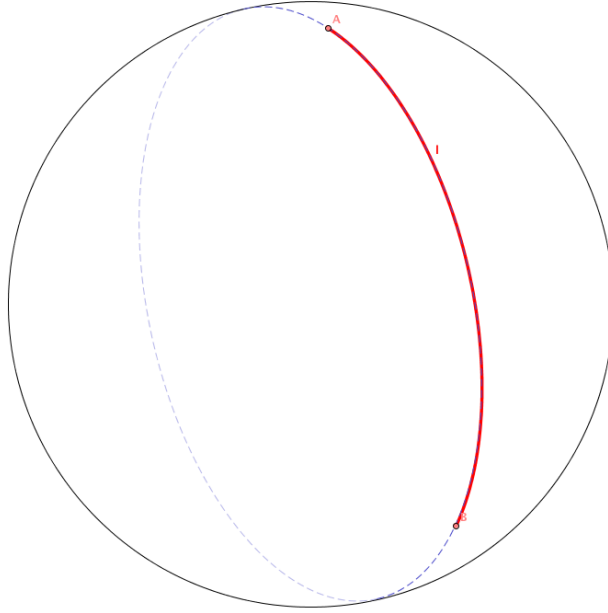
Figure 1.2: The shortest path l between two points A and B on a sphere is along an arc of great circle.
