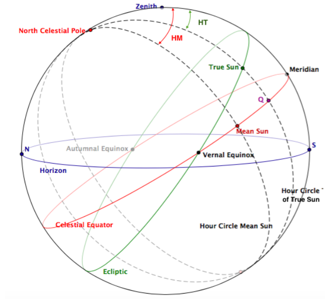
Figure 1.22: A mean Sun is defined in the celestial equator, that moves in uniform motion in right ascension over the year, and in hour angle in diurnal motion. The point Q is the projection of the true Sun on the celestial equator. The difference between the Hour Angles of the true Sun ( H_T ) and the Mean Sun ( H_M ) is the Equation of Time ( E ), E = H_T - H_M .
