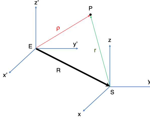
Figure 1.31: Translation to barycentric coordinates.
